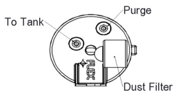
Carbon Canister Detail
