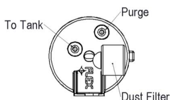
Carbon Canister Detail
